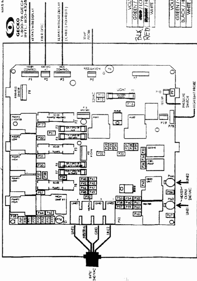
PUMP #1 CONNECTOR
